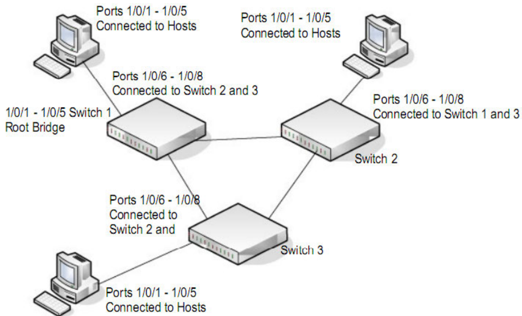
Figure 2. MSTP example configuration
