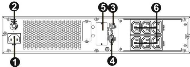
IEC Type
