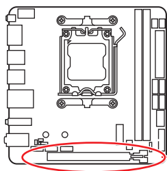
PCI_E1: PCIe 4.0 x16 (From CPU)
